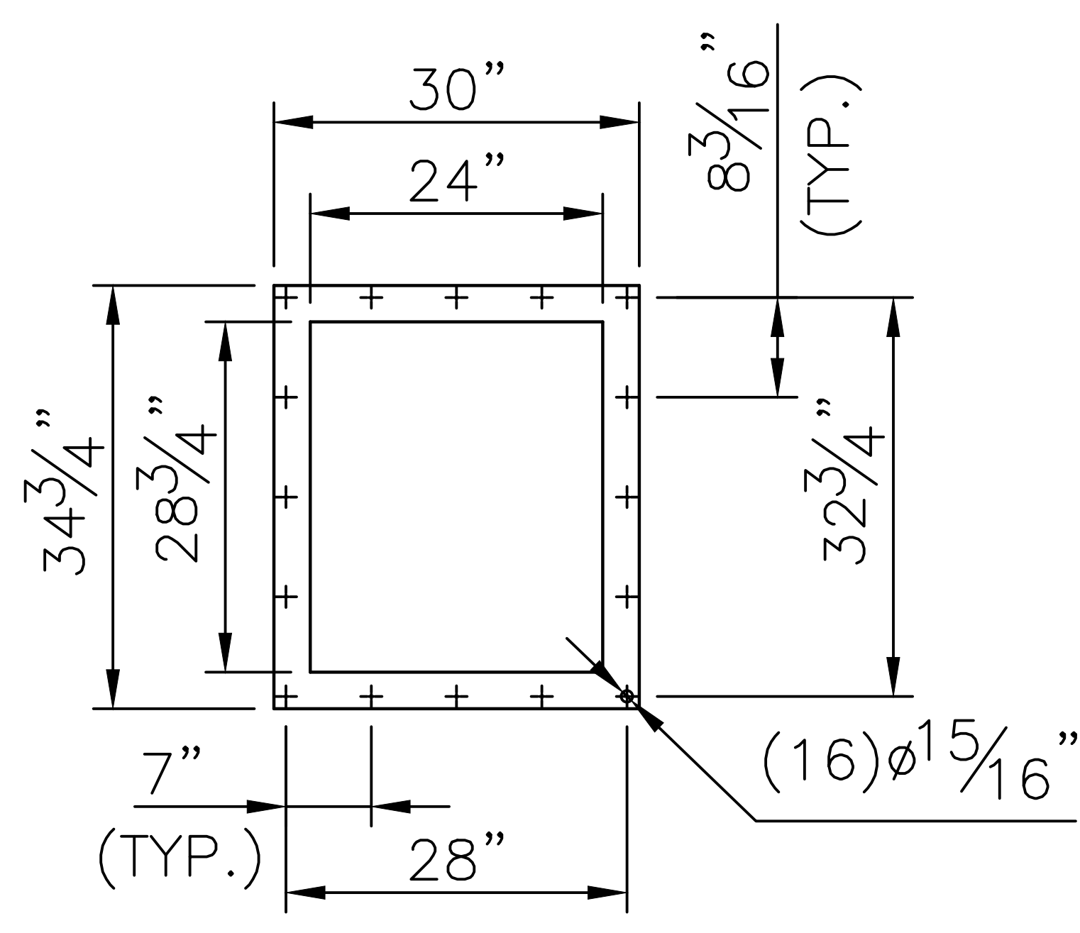
INLET FLANGE
